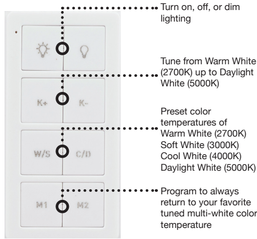
TandemLED wireless controller
