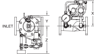
Pilot System Dimensions
