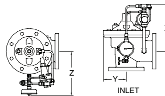
Angle Pilot System Dimensions
